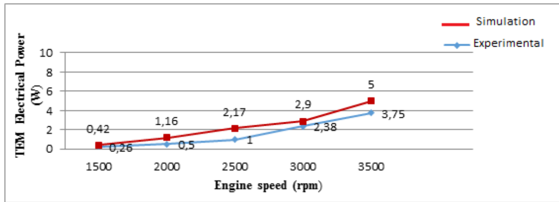
Figure 6. The obtained electrical output data
