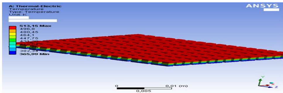
Figure 5. The temperature distribution of the TEM system of the operation situation of the engines 1500 rpm (a), 2000 rpm (b), 2500 rpm (c), 3000 rpm (d) and 3500 (e) rpm
