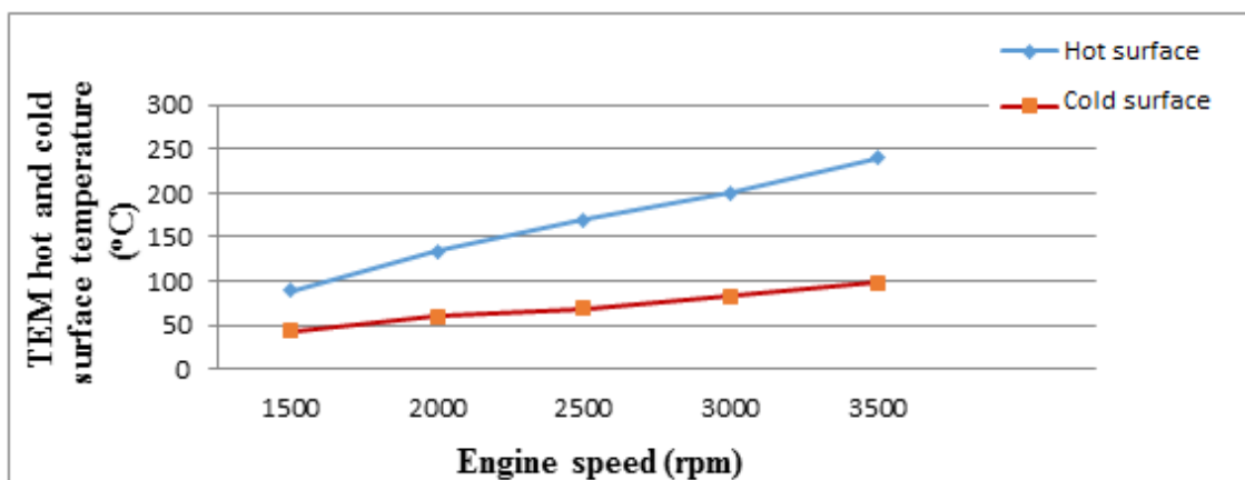
Figure 4. The temperatures on the surface of TEM
